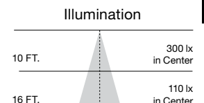
Beam Angle : 25°
