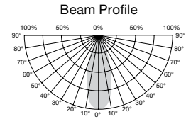
Beam Angle : 40°
