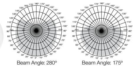
Candle Beam Profile
